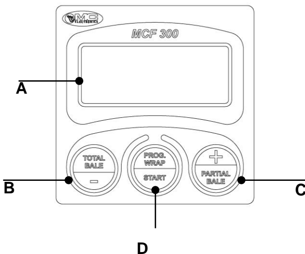
Figure 5. Vue frontale.
